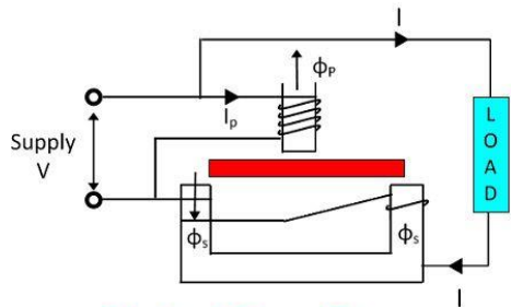
Working of Energy Meter
