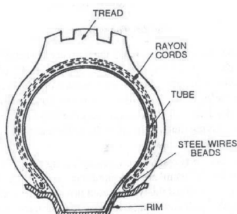
Fig. Traditional Tube Tyre
