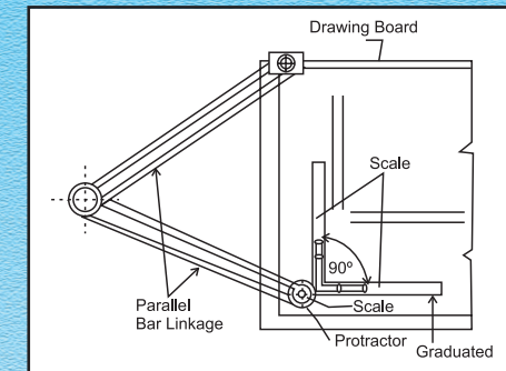
Drawing Sheet Fig.1.30.2
