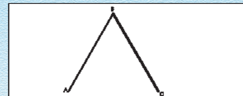
ABC is the vertex or apex of the angle ABC Fig. 1.7.9
